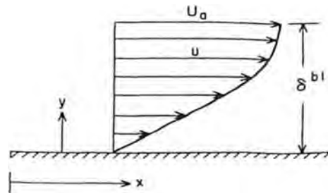
FIGURE 9.2 Boundary layer created at the surface of a stationary plate over which a fluid is moving with an ambient velocity U_a . At some distance x from the edge of the plate and at some vertical distance y from the surface of the plate, the velocity of the fluid u equals U_a . The distance y at which the local velocity equals 90% of the ambient velocity is the thickness of the boundary layer.
