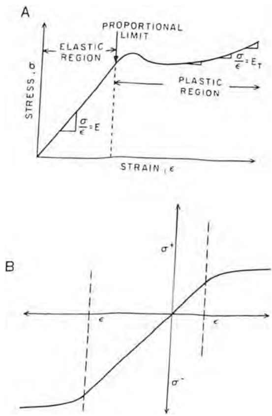
FIGURE 2.8 Linear elastic behavior and plastic behavior as revealed by a material's stress-strain diagram: (A) Linear elastic behavior is evinced by an initial linear region on the stress-strain diagram. The slope of this portion of the stress-strain diagram is called the elastic modulus (or Young's modulus), symbolized by E : that is, E = \sigma/\epsilon . The portion of the stress-strain diagram where stress and strain are proportionally related to one another by the constant E is called the elastic region. The plastic region of the stress-strain diagram is nonlinear, and the ratio of stress to strain varies within this region depending on where the slope is measured. The slope measured anywhere on the stress-strain diagram is called the tangent modulus ( E_T ). The proportional limit is the stress level below which elastic behavior is manifest. (B) The proportional limits of the same material measured under tensile and compressive stress ( \sigma^+ and \sigma^- , respectively) may not be equivalent even if the elastic moduli measured in tension and compression are equivalent.
