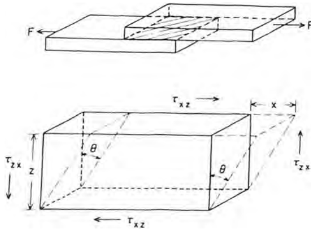
FIGURE 2.4 Shear stress \tau is calculated by dividing the shear force ( F ) applied to a material by the area through which it operates: (A) Two rectangular elements joined by the crosshatched area, \tau = F/A . (B) The shear stress components \tau_x and \tau_z , have a corresponding shear strain y as illustrated by a rectangular element (solid outline) distorted into a parallelepiped (dashed outline) by a shear force, applied tangentially (in the xz plane). The figure illustrates pure shear. The magnitude of the shear strain can be calculated from the translation angle of the specimen's corners \theta : \gamma = \tan \theta = x/z .
