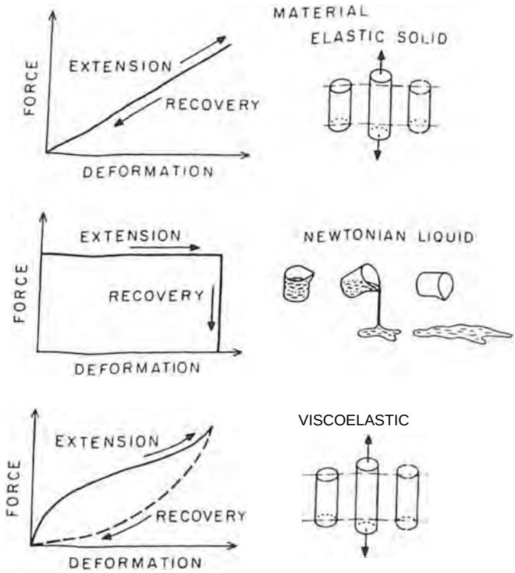
FIGURE 2.13 Force-deformation diagrams of a linear elastic solid, a Newtonian liquid, and a viscoelastic material. Linear elastic solids recover all of their deformations when applied forces are removed provided their proportional limits are not exceeded; that is, deformations are recoverable within the elastic range of behavior. Newtonian fluids do not recover any of their deformations when an applied force is removed. Viscoelastic materials recover deformations gradually when applied forces are removed.
