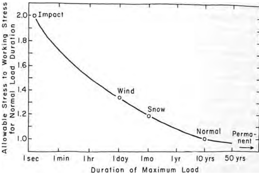
FIGURE 7.13 Design factor ("safety factor") for a vertical wooden column plotted as a function of the duration of maximum load. The design factor is taken as the ratio of the allowable stress to working stress for the normal load duration. The allowable stress refers to the maximum stress the column is designed to withstand. Working stress refers to the stress calculated to result from the static loading of the structure (based on the "normal" load duration). As the duration of the maximum load experienced by a column decreases, the design factor increases. Wooden columns that are expected to experience impact load durations (2 sec or less) have the highest design factor (which equals 2); wooden columns that sustain permanent load durations (fifty years or more) are designed with the lowest design factor (which equals 0.9). See text for further details.
