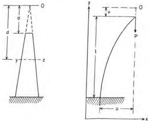
FIGURE 7.7 Linearly tapered beam for which changes in the second moment of area can be calculated. The second moment of area for any transverse plane y - z at a distance d from origin of taper O can be calculated based on a power function and the second moment of area at the free end of the beam (at distance a from the origin of taper). The less the degree of taper the less the tip load P required to cause the beam to deflect from the vertical (shown to the right of this figure).
