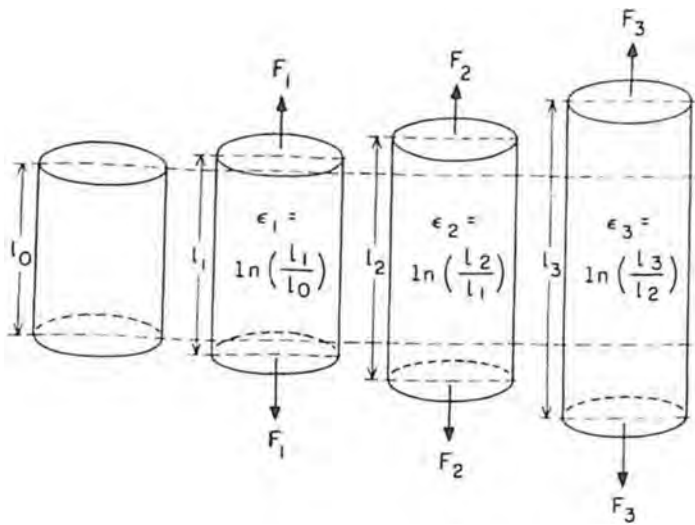
FIGURE 2.5 True strains \epsilon , calculated for a cylinder subjected to increasing uniaxial tension resulting from the application of tensile forces with increasing magnitudes ( F_1 , F_2 , and F_3 ). As a result of the tensile forces, the cylinder extends in length and contracts in girth. The true strain is the natural logarithm ( \ln ) of the extension ratio. The extension ratio is the ratio of the magnitude of the instantaneous dimension to that of the previous dimension (e.g., l_1/l_0 which is the extension ratio of the increase in length due to the application of the tensile force F_1 to the original length).
