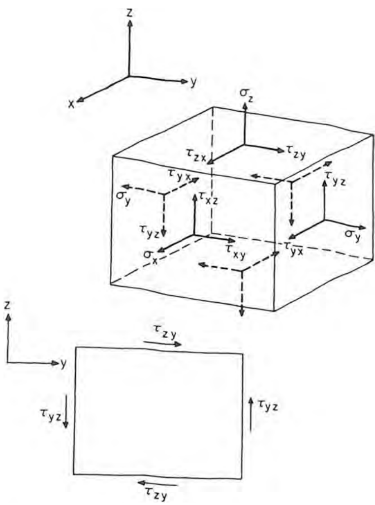
FIGURE 2.1 Normal and shear stresses within a cubical element of a material with depth x , width y , and length z . Three normal stresses, \sigma_x , \sigma_y , and \sigma_z , operate perpendicular to the three orthogonal axes of the element. Parallel sides of the cubical element have equivalent magnitudes of normal stress. Six shear stresses, \tau_{xy} , \tau_{yx} , \tau_{yz} , \tau_{zy} , \tau_{xz} , and \tau_{zx} , operate parallel to the surfaces of the cubical element. The "shear stresses operating perpendicular to the line of intersection of perpendicular sides of the cubical element are equivalent: \tau_{xy} = \tau_{yx} , \tau_{yz} = \tau_{zy} , \tau_{xz} = \tau_{zx} . Therefore only six stress components ( \sigma_x , \sigma_y , \sigma_z , \tau_{xy} , \tau_{yz} , \tau_{xz} ) are required to specify the internal forces (= stresses) generated within the element as a result of the application of an external force. (From Timoshenko and Goodier, Theory of Elasticity [1970], fig. 3, reproduced with permission of McGraw-Hill, Inc.)
