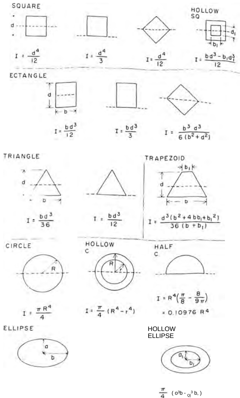
FIGURE 3.3 Formulas for the second moment of area / for members with different cross-sectional geometries. The geometry of each member is indicated by a single representative cross section. The formula for the second moment of area, even for the same geometry, depends on the plane of bending, which is shown by a dashed line in each drawing. The second moment of area always has units of length raised to the fourth power, since it is computed as the sum of the products of each infinitesimally small area A and the square of the distance d of the area from the centroid axis
