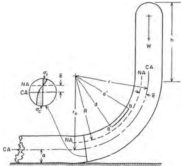
FIGURE 7.6 Relations among mechanical parameters for a curved beamlike plant axis resting on a substrate and bearing a weight at its tip. The transection to the left of the figure illustrates the distribution of tensile \sigma_t and compressive \sigma_c bending stresses relative to the centroid axis (CA) and neutral axis (NA). The tensile stresses develop within the upper, concave surface of the plant axis because the upward bending of the beamlike axis is the result of growth and gravity exerts a force on the vertical biomass. Thus compressive stresses develop on the convex surface of the beamlike organ. This spatial distribution of stresses is the reverse of the stress distribution that would develop in a beam forcibly bent into the shape achieved here by growth. The NA lies a distance e from the CA. The bending stresses developed within the curved beam depend on the radius of curvature R , the weight supported by the beam W , the uncurved, vertical height of the beam h , and the way the radius of curvature changes over the curved span of the beam. For further details, see text. (From Niklas and O'Rourke, 1982.)
