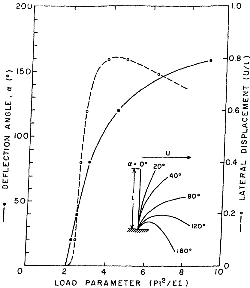
FIGURE 3.6 Predicted and observed changes in the tip deflection angle ( \alpha ) and in the ratio of the lateral displacement ( U/l ) to leaf length ( l ) plotted as a function of the load parameter ( Pl^2/EI ) of a progressively bending chive leaf (see insert). The predicted changes are plotted as lines; observed values are plotted as data points (solid circles and open circles). The load parameter is a dimensionless ratio that relates the product of the load applied ( P ) at the free end of a beamlike structure (the chive leaf) and the square of the beam length ( l ) to the flexural stiffness ( EI ). As the load parameter increases, the beam experiences greater deflections from the vertical. See text for further details. (Data from Niklas and O'Rourke 1987.)
