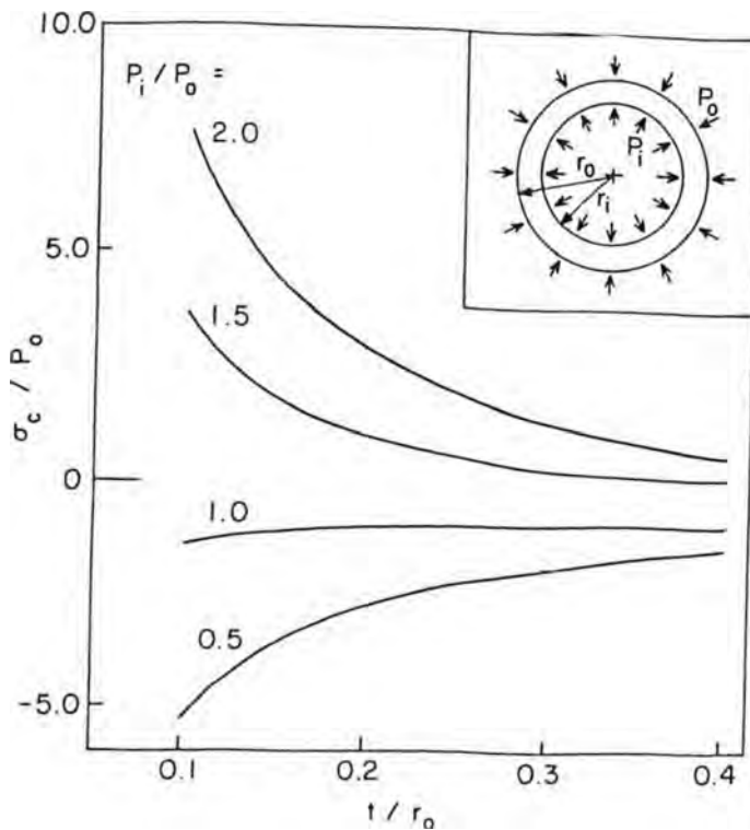
FIGURE 5.4 Theoretical relation among circumferential (hoop) stresses ( \sigma_c ) generated within a tubular cell with wall thickness t and outer radius r_o , subjected to an inner (turgor) and an outer pressure P_o . (The inserted diagram to the upper right of the graph shows a cross section through the cylindrical cell wall with an inner radius of r_i .) The relations among pressure, circumferential stress, and cell wall dimensions are expressed in terms of three dimensionless ratios P_i/P_o and t/r_o . The ratio of circumferential stress to the external pressure ( \sigma_c/P_o ) is plotted as a function of the ratio of cell wall thickness to cell wall outer radius ( t/r_o ) for four different ratios of turgor to external pressure ( P_i/P_o ). As the thickness of the cell wall increases (as t/r_o increases), the predicted ratios of circumferential stress to the external pressure ( \sigma_c/P_o ) converge for any ratio of turgor to external pressure ( P_i/P_o ); for any wall thickness ( t/r_o is a constant), the ratio of circumferential stress to external pressure ( \sigma_c/P_o ) increases as P_i/P_o increases. These relationships indicate that when the wall thickness is equal to or exceeds roughly 20% of the cell radius, the turgor pressure plays little or no role in determining the circumferential stresses within the cell wall. (From Niklas 1989c.)
