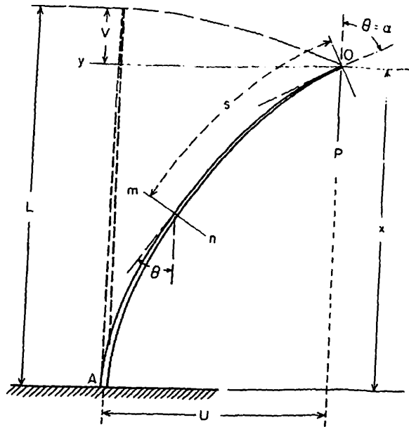
FIGURE 3.5 Large bending deflections of a beam anchored at one end (A) and subjected to load P at its free end (O). Before the application of the load, the beam is perfectly vertical (dashed outline to the left). With the application of the load, the beam undergoes vertical ( V ) and horizontal ( U ) displacements. A bending angle \theta is defined at any cross section through the beam (along the plane m - n ) at a distance, measured as a function of the arc length s , from the tip of the beam. The tip deflection angle ( \theta - \alpha ), in conjunction with equations from the Elastica (see text), is used to compute the relation among beam length L , flexural stiffness EI , and the magnitude of the load P .
