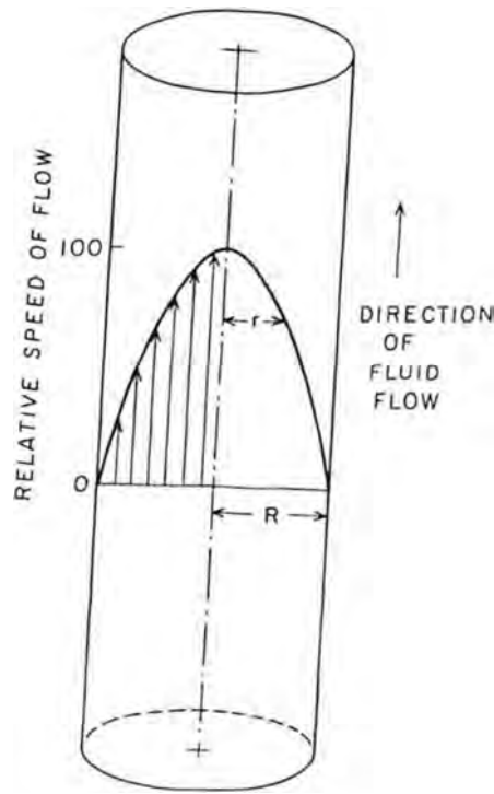
FIGURE 4.11 Diagram of fluid (liquid) flow through a vertical capillary tube. The direction of flow is from the bottom to the top of the figure. The velocity profile of the flow is parabolic; the maximum speed of flow is at the center of the capillary tube ( r = 0 ), while the speed of flow of the liquid at the liquid-tube wall ( r = R ) interface is zero.
