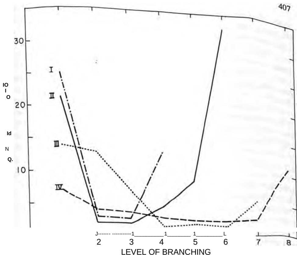
FIGURE 8.10 Loading parameter ( PP/EP ) of Psilotum nudum plotted as a function of the level of branching in four (I-IV) vertical trusses of the sporophyte generation. The basalmost branch element (level 1) and highest level of branching in each truss have higher loading parameters than intermediate branching levels. However, as the size of the truss increases (measured by the number of the levels of branching) from truss I to truss IV, the loading parameter of level 1 decreases, indicating that the flexural stiffness of the subtending branch element has increased relative to the load (biomass) it must support. (From Niklas 1990c.)
