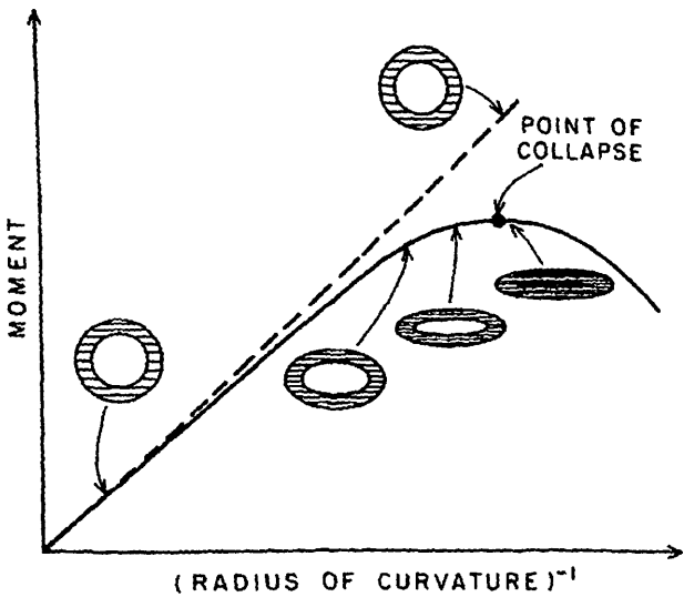
FIGURE 7.10 Bending moment plotted as a function of the reciprocal of the radius of curvature ( 1/r ) for two hollow cylindrical beams made of different materials. A cylinder composed of a relatively stiff material will resist ovalization (dashed line) when subjected to the same bending moments as a cylinder made of a less stiff material, which will undergo Brazier buckling (solid line) owing to the progressive ovalization of its originally circular cross section. A beam that resists ovalization has a linear moment-curvature relation; a beam that undergoes Brazier buckling has a nonlinear relation between moment and curvature. At some bending moment (the critical bending moment) ovalization leads to Brazier buckling, at which point the beam collapses.
