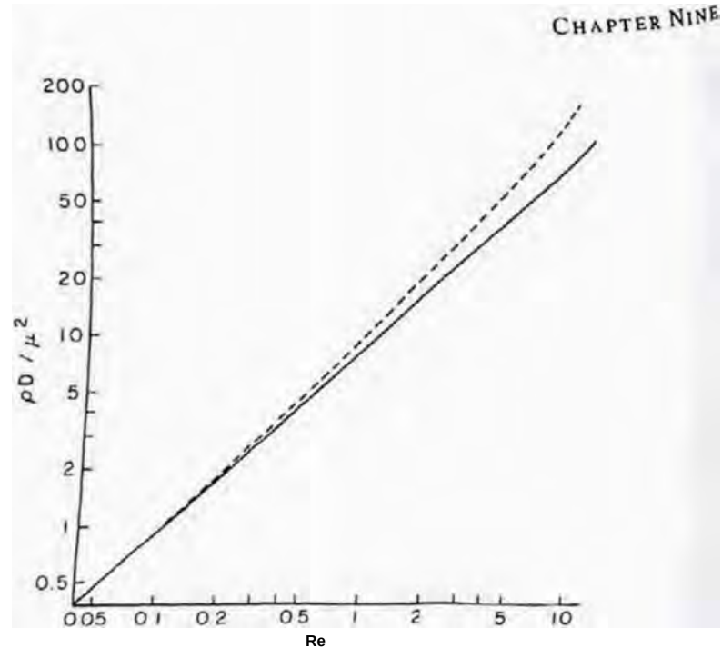
FIGURE 9.5 Drag on a sphere (expressed as the ratio of the product of density and drag to the square of dynamic viscosity: \rho D/\mu^2 ) plotted as a function of low Reynolds number ( Re ). Dashed line indicates empirical observations; solid line calculated from Stokes's law (see text, eq. 9.13).
