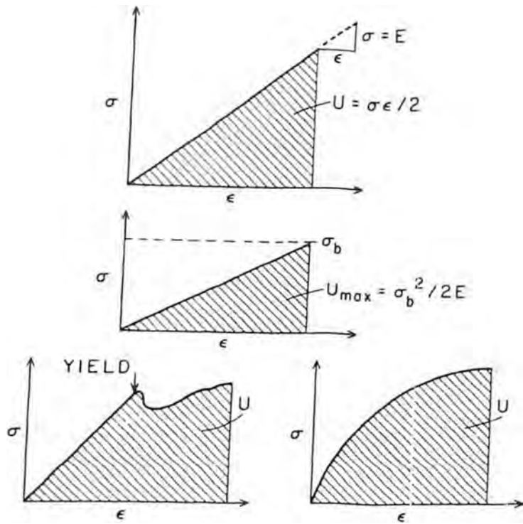
FIGURE 2.20 Relation between maximum strain energy and strength. Strain energy ( f ) is the energy stored within a material as it is loaded. For a linear elastic nonductile material, U is computed from the formula U = CFE/2 = cr^2/2E = E\epsilon^2/2 per unit volume of material. The maximum strain energy ( t_{max} ) can be computed from its elastic modulus and its breaking stress cr_b ; = u^2/2E . For a ductile or plastic material the strain energy must be computed empirically from the area under the stress-strain diagram. The strength of a material is the maximum stress it can sustain before it breaks or begins to yield. For a material, strength has the same units as stress (force per area).
