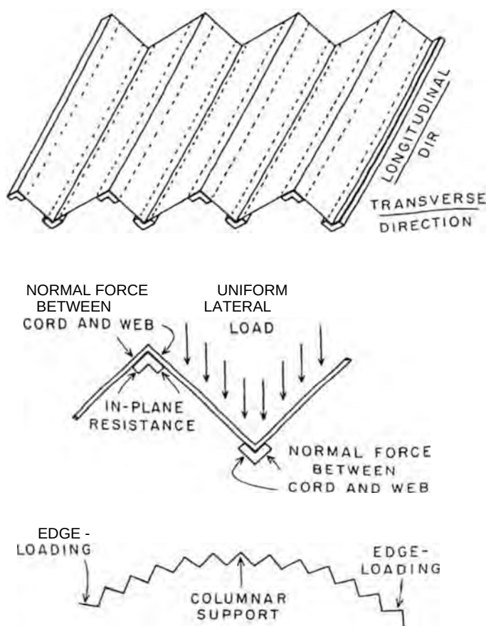
FIGURE 7.14 Cord-web model for some leaves. The leaf can be considered to operate mechanically as a series of longitudinally aligned beamlike cords interconnected by a relatively thin webbing. The uniform lateral loading of the webbing generates normal forces between the cord and web elements. When such a structure is supported by a column, it undergoes edge loadings that cause its unsupported span to deflect. The “column” could be a more robust “midrib” running the length of the corrugated cord-web shell; the edge loadings could simply be the weight of the cord-web structure on either side of the midrib.
