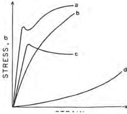
FIGURE 2.11 Representative stress-strain diagrams for four different types of materials: Linear elastic material undergoing plastic deformations and strain hardening (a); non-linear elastic material with a decreasing tangent modulus (b); linear elastic material undergoing plastic deformations and strain softening (c); and nonlinear elastic material with an increasing tangent modulus (d).
