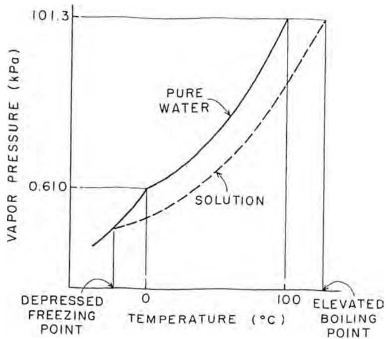
FIGURE 4.3 Vapor pressure of pure water and of a solution of water plotted as a function of temperature. Adding solutes to pure water depresses the freezing point of the solution compared with that of pure water. Adding solutes to pure water elevates its boiling point.
