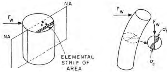
FIGURE 7.11 Bending of a beamlike plant axis owing to the lateral force exerted on it by wind ( F_w ). Lateral wind loading results in a bending moment, placing tissues in either tensile or compressive stress that increases in magnitude as a function of the distance x from the neutral axis NA. Within each transection, the intensity of both the tensile and the compressive stresses that develop in each elemental strip aligned parallel to the plane of bending increases as a function of the distance x of the elemental strip from the neutral axis. For further details, see text.
