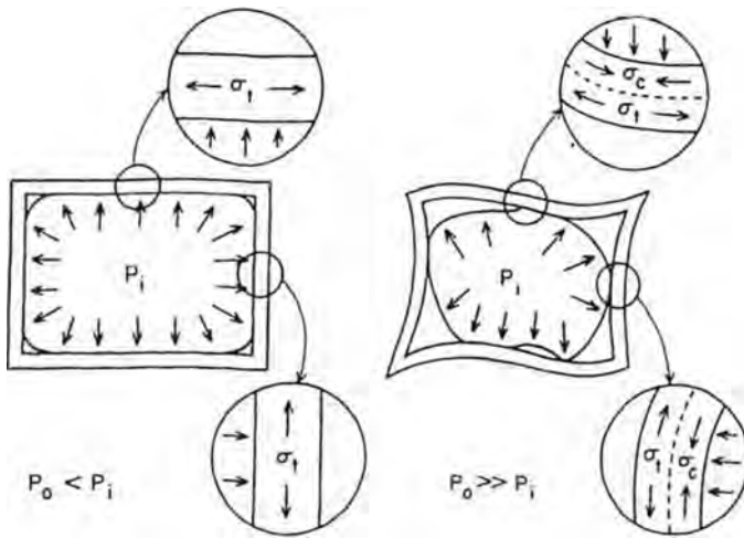
FIGURE 6.3 Theoretical effect of turgor pressure ( P_i ) on the distribution of tensile (ct,) and compressive (cr,) stresses within the cell wall of a hydrostatic (thin-walled) cell. When fully inflated and appressed to the cell wall, the protoplast will place the cell wall in overall tensile stress and will restrain it from bending when a load is applied externally (diagram to left of figure). When the internal turgor pressure of the cell drops below the external pressure, the protoplast deflates and may pull away from the cell wall (highly exaggerated in the diagram to the right). When an external force is applied to the cell, the cell wall is free to bend and buckle, and it experiences both compressive and tensile stresses as it deforms.
