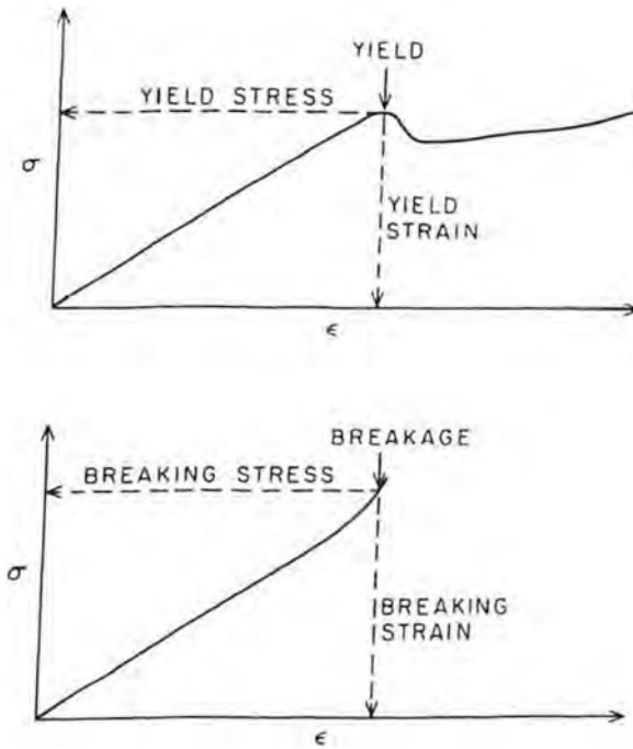
FIGURE 2.18 Stress-strain diagrams for a linear elastic ductile material (upper diagram) and a linear elastic brittle material (lower diagram). Ductile materials undergo plastic deformation beyond their proportional limits when the yield stress is achieved in their loading cycle. Brittle materials break when their proportional limits are exceeded. The stress level at which breakage occurs is called the breaking stress.
