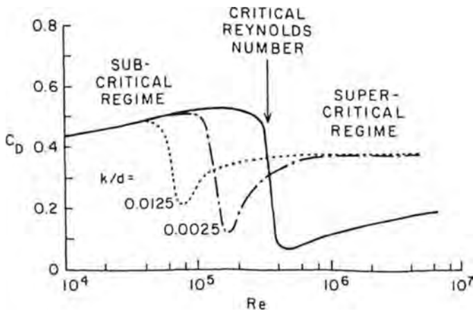
FIGURE 9.6 Relation between the drag coefficient C_D and the Reynolds number for a sphere with a smooth surface (solid line) of diameter d and for two spheres with roughness elements (dotted and dashed lines) with two different heights k . The critical Re is seen as a sharp decrease in C_D .
