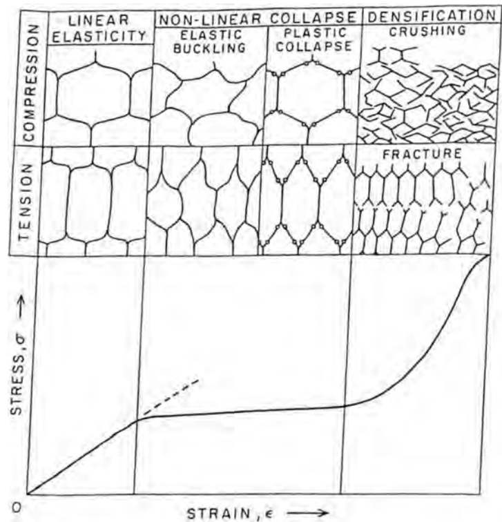
FIGURE 6.7 Geometric distortions with a typical honeycomb cellular solid subjected to compression (above) and a typical stress-strain diagram under compressive loading (below). Transections through a honeycomb cellular solid reveal the types of geometric distortions that are likely to occur when the solid is subjected to compression. These distortions can involve elastic buckling, plastic collapse (the likely locations of plastic hinges are shown as small circles), or crushing (in compression). The stress-strain diagram resulting when a cellular solid is placed in compression typically shows three regions (linear elasticity, nonlinear collapse, and densification). The features of the stress-strain diagram result from deformations occurring within the cellular voids of the solid (upper panel). (From Niklas 1989c.)
